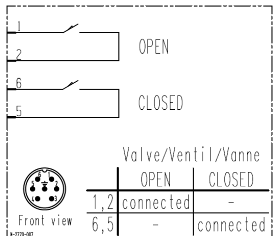
Wiring diagram
